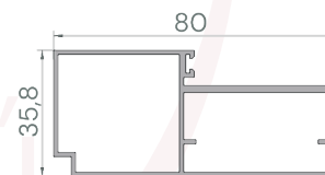
ALN-373613
